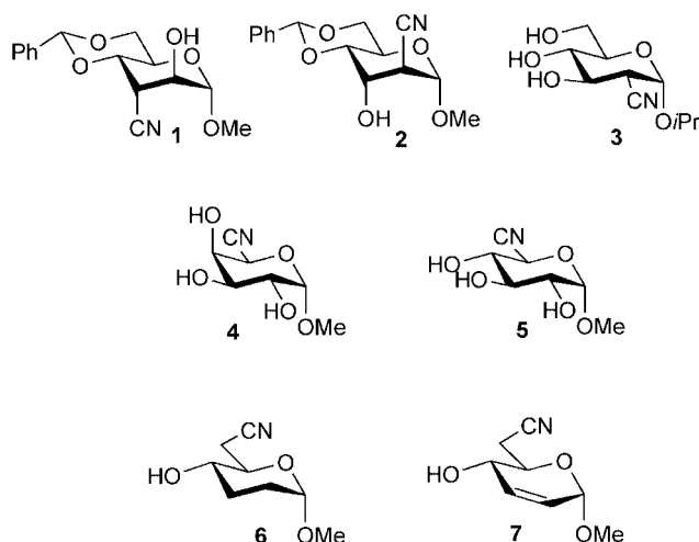
Figure 1. Cyanopyranosyl derivatives 1–7.
