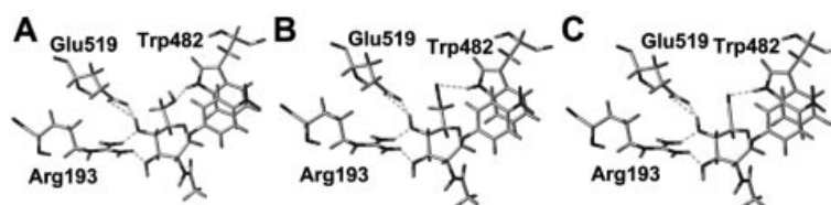
Figure 3. Substrates A) 12a , B) 9 and C) 8 docked into the active site of the β-N-acetylhexosaminidase from A. oryzae CCF 1066. Hydrogen bonding (in green) to glutamic acid 519, arginine 193 and tryptophan 482 fixes the glycosides. The π-electron system of the aromatic ring of the p -nitrophenyl group is stabilized by aromatic stacking with tryptophan 482.
