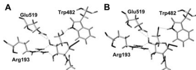
Figure 4. Substrates A) 12b and B) 10 docked into the active site of the β-N-acetylhexosaminidase from A. oryzae CCF 1066. Hydrogen bonding (in green) to glutamic acid 519, arginine 193 and tryptophan 482 fixes the glycosides. The azido group is depicted as a blue stick.
